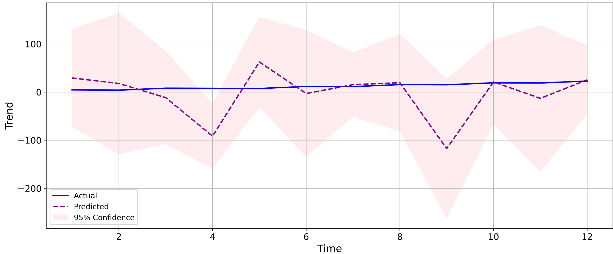
Malvertising-ALL - Validation
